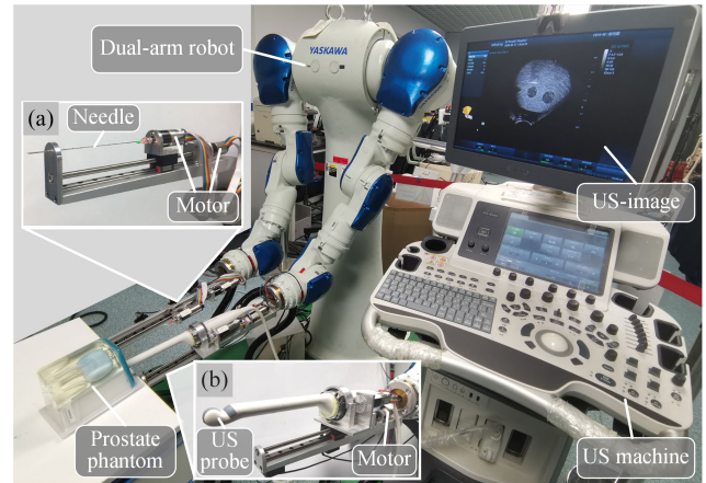
Fig. 2. US-guided dual-arm robotic system for prostate brachytherapy. (a) Needle end-effector. (b) US probe end-effector.
