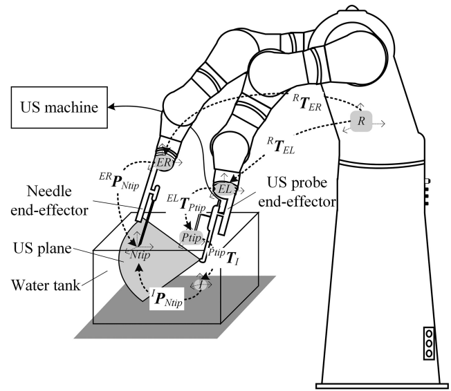
Fig. 4. Transformations involved in the US-guided dual-arm robotic brachytherapy system. ( R : Robotic base frame. ER : End-flange frame of the right robotic arm. EL : End-flange frame of the left robotic arm. Ntip : Needle-tip frame. Ptip : US probe-tip frame. I : US image frame.).
