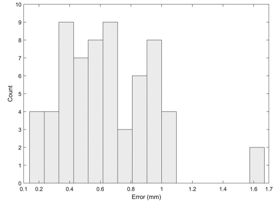
Fig. 11. Distribution histogram of 64 experimental errors (an example of ICP algorithm).
