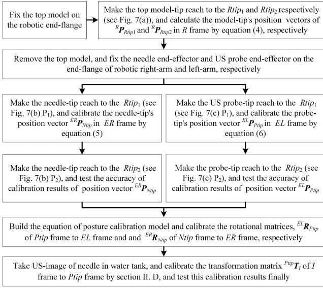
Fig. 9. Overall calibration procedure. ( R : Robotic base frame. ER: End-flange frame of the right robotic arm. EL: End-flange frame of the left robotic arm. Ntip: Needle-tip frame. Ptip: US probe-tip frame. I : US image frame.).
