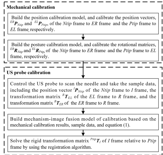
Fig. 5. Overall framework of the proposed calibration approach. ( R : Robotic base frame. ER : End-flange frame of the right robotic arm. EL : End-flange frame of the left robotic arm. Ntip : Needle-tip frame. Ptip : US probe-tip frame. I : US image frame.).
